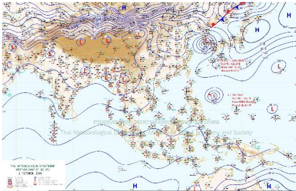
Figure 1: Weather map for 02 nd Oct 2019
