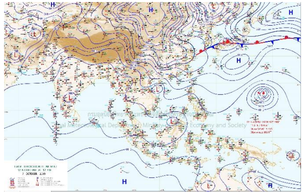
Figure 2: Weather map for 07 th Oct 2019
