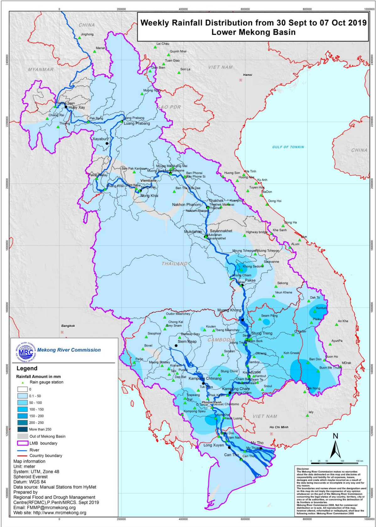
Figure 3: Weekly Rainfall Distribution over the LMB from 01 st to 07 th Oct 2019
