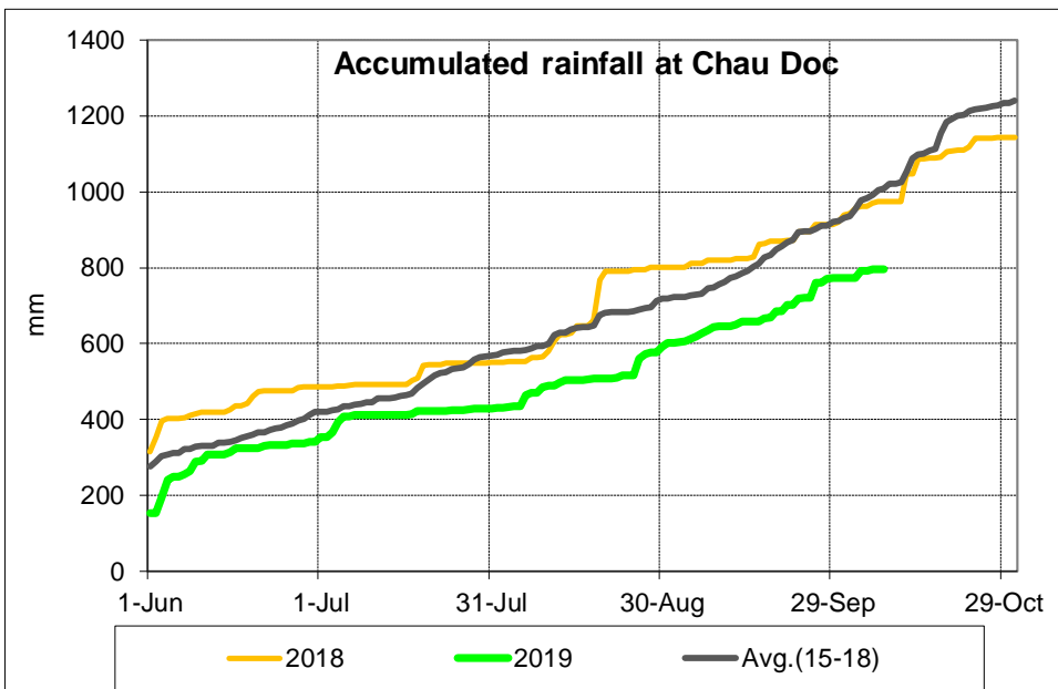
Figure 4: Accumulated Rainfall up to 08 th October to 2019 in specific stations over the LMB
